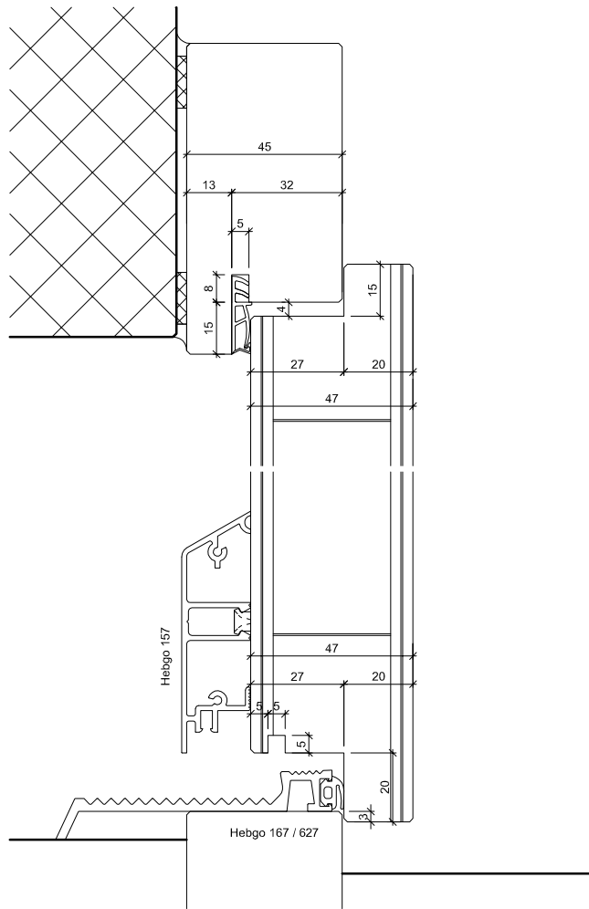
Detail B-B
