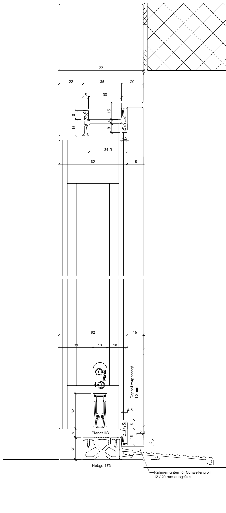
Detail B-B
