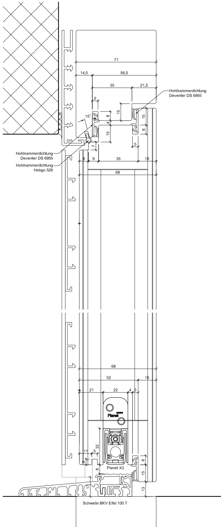
Detail B-B
