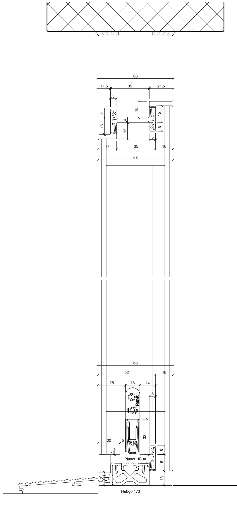
Detail B-B
