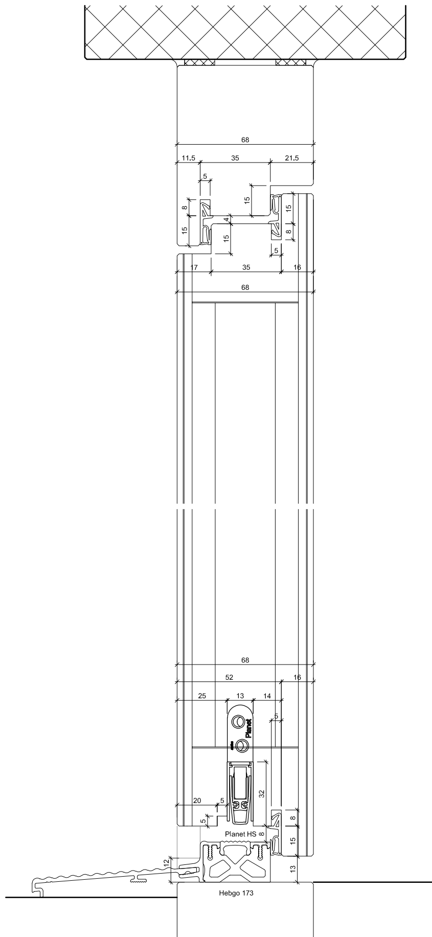
Detail B-B
