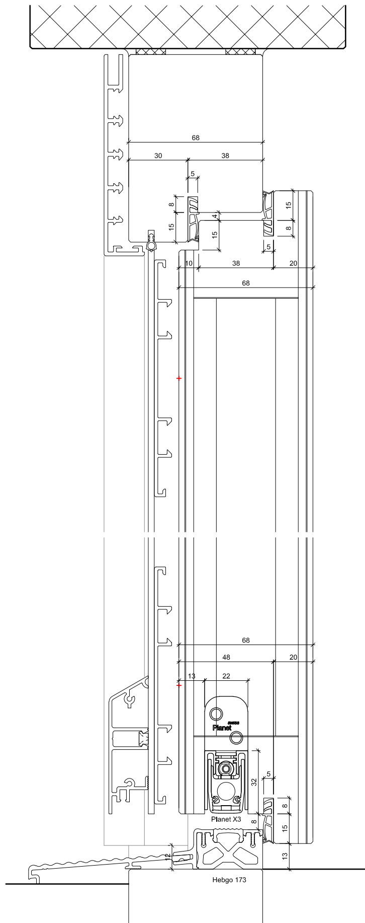
Detail B-B
