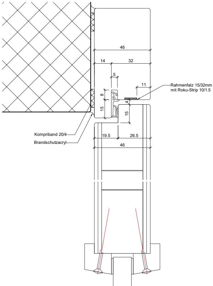
B-B Detail oben
