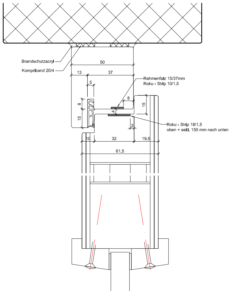
B-B Detail oben
