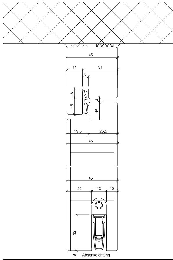
Detail B-B
